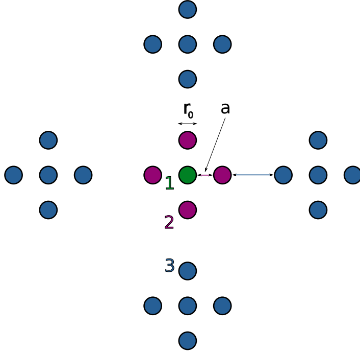
Figure 2: Diversity recursion.
